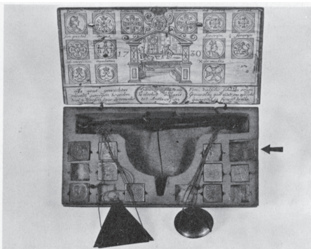
Fig. 89. Weight and scale box made by J. F. Wolschot, Antwerp, dated 1730. The label shows a man using the gold scale and indicates which weight is for which coin. The gold weights are in their recesses; the scale has one round and one triangular pan. The arrow indicates a small container for grain weights (lid missing).
